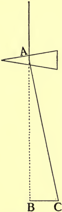
FIG. 200.—Deflection caused by a prism.
